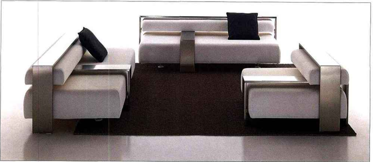
Ensemble MAZE
